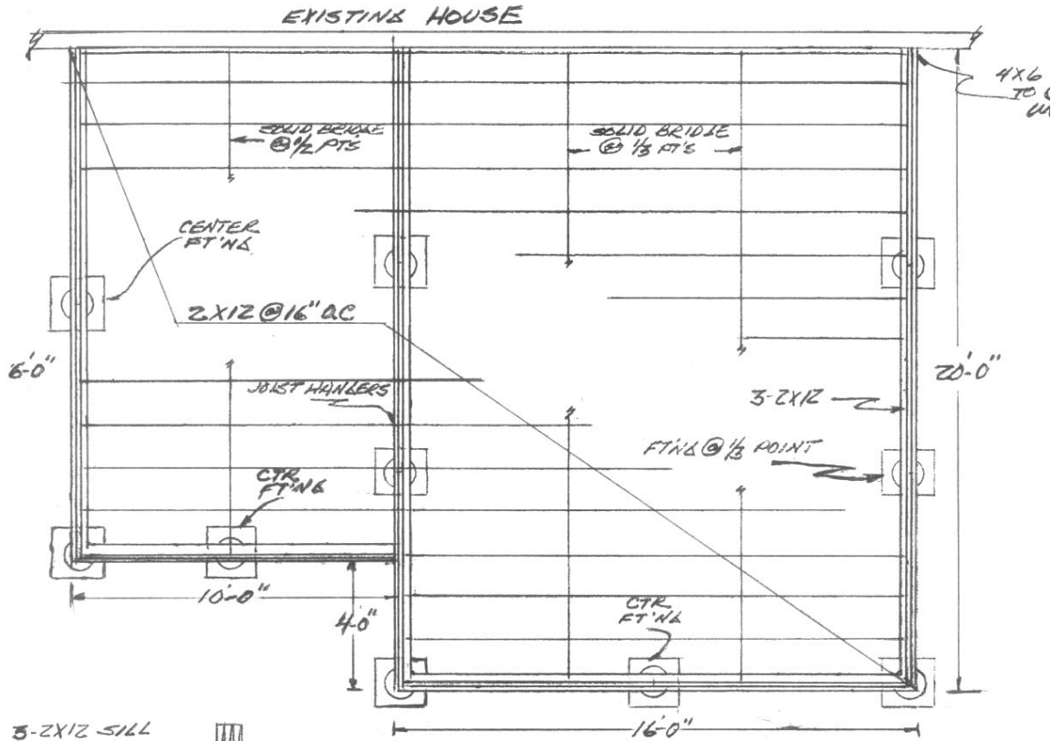
FOUND & 1ST FLR FRM PLAN SCALE: 1/4" = 1'-0"
