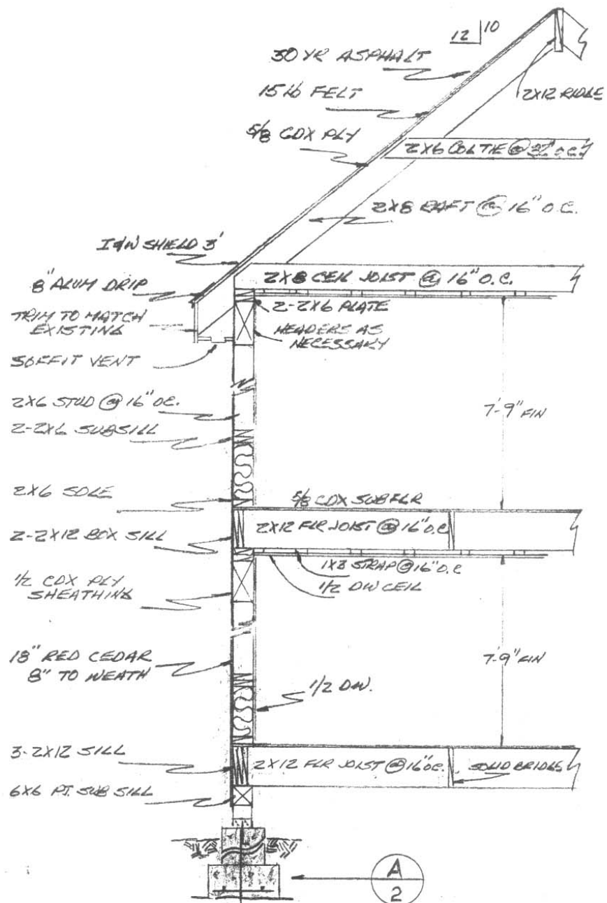
TYPICAL WALL SECTION SCALE 3/8" = 1'-0"
